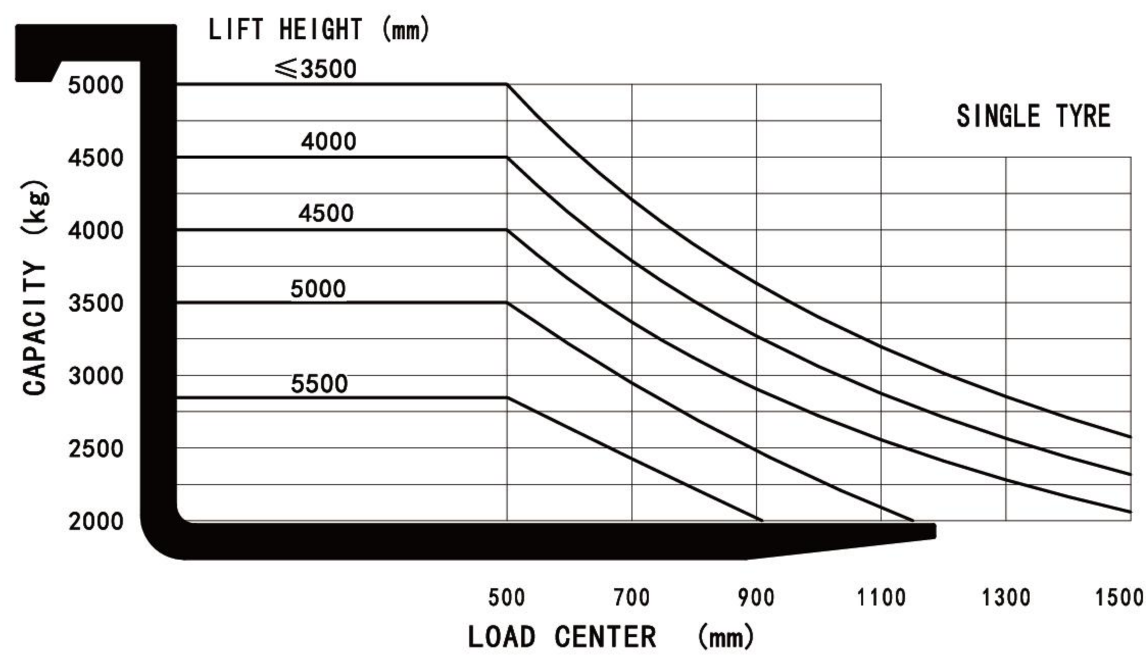
CAPACITY CHART
